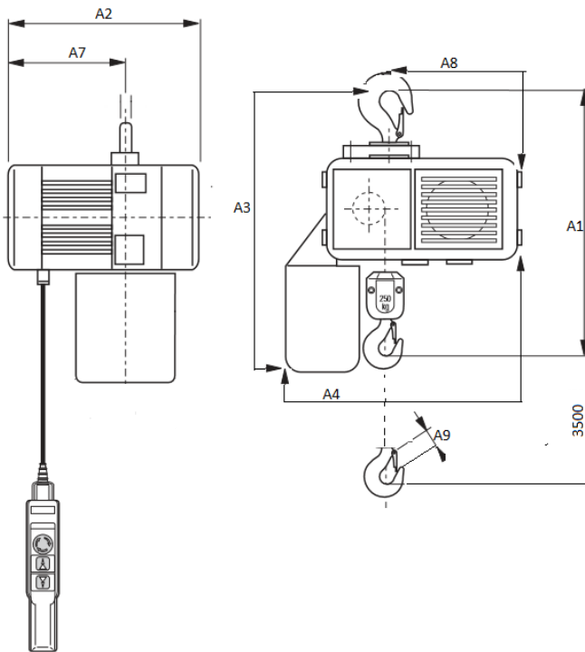
Standard Chain Hoist with Hook
