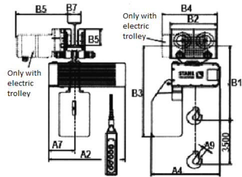
Hoist with Trolley
