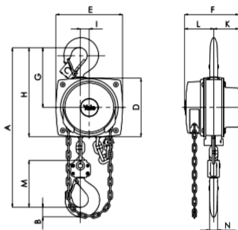
Yalelift 360 ATEX Rated 1/4 tonne, single fall
