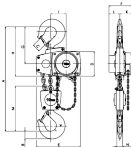
Yalelift 360 ATEX Rated 5 to 6 tonne, three fall
