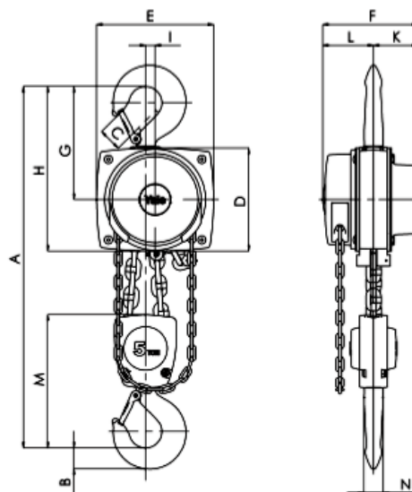
Yalelift 360 ATEX Rated 3 to 4 tonne, double fall
