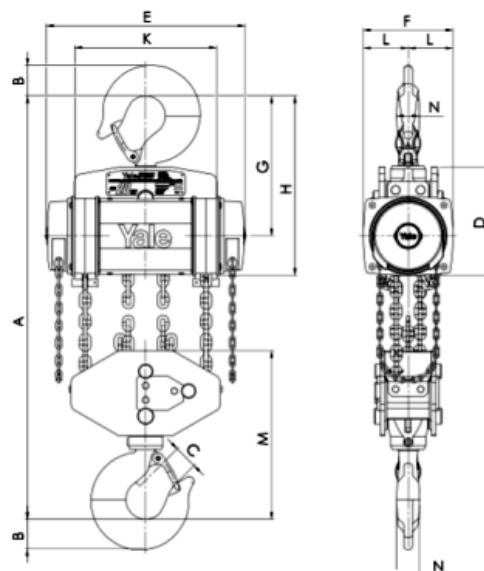
Yalelift 360 ATEX Rated 8 to 12 tonne, six fall
