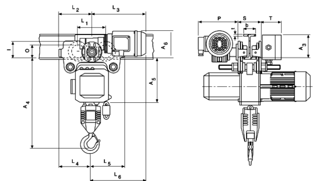
Model CPE/CPEF with integrated electric trolley
