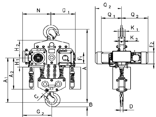
Model CPE/CPEF 100-2 with suspension hook, 10000kg
