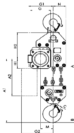
Model CPE/CPE/F 75-1, 6 with suspension hook, 7500kg
